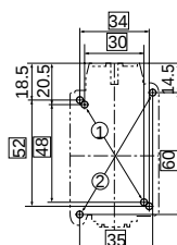
Panel drilling
