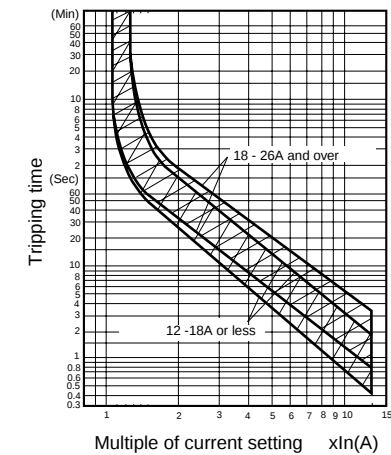
TR-3N/3
