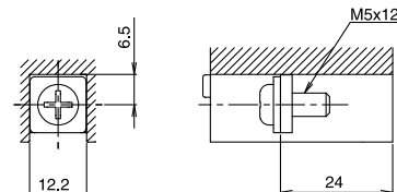
Terminal section
