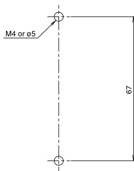
Panel drilling
