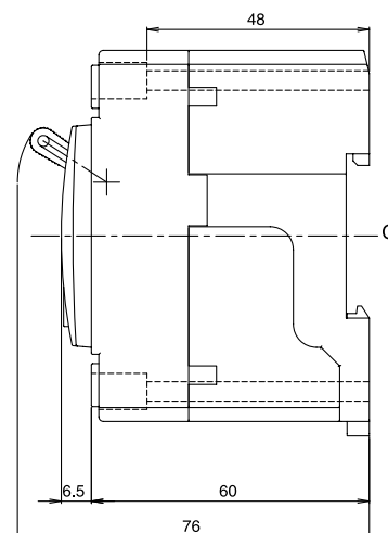
Terminal section
